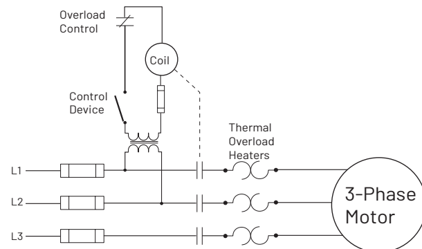
Figure 4-8: Low Voltage Control
