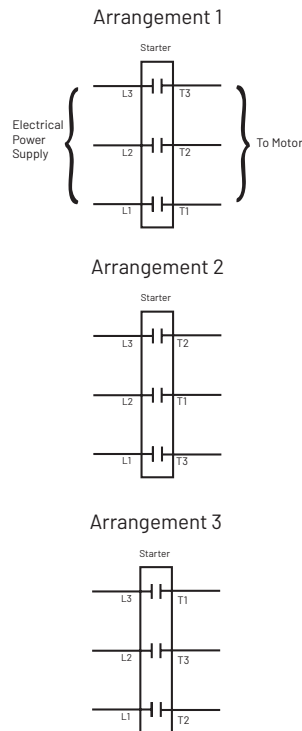
Figure 4-11: Example of Three-Phase Current Unbalance
