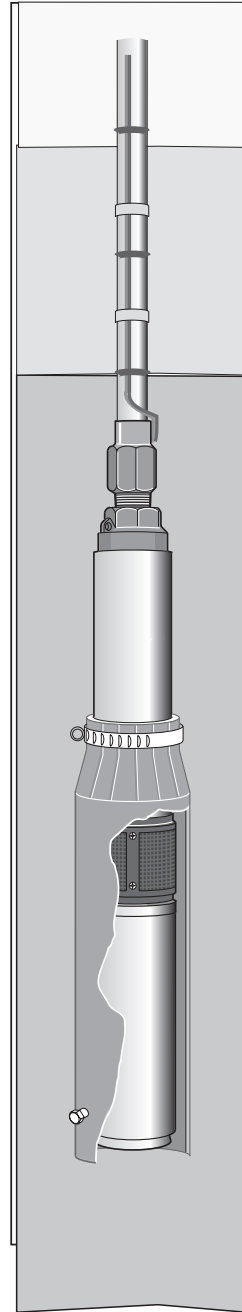
Figure 5-2: Flow Inducer Sleeve
