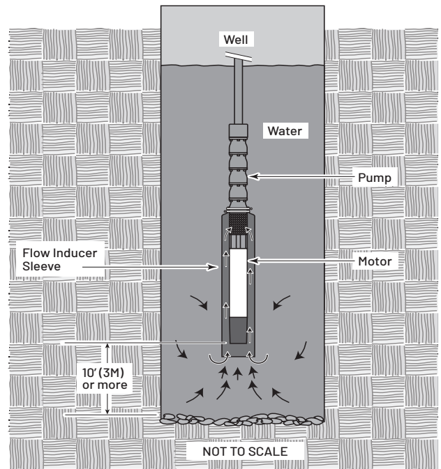
Figure 6-3: If flow past motor is less than .5 fps (0.15 mps), install a flow inducer sleeve as shown. Flow must be at least .5 fps (0.15 mps) for adequate motor cooling. The flow inducer sleeve should not touch the side of the motor.
