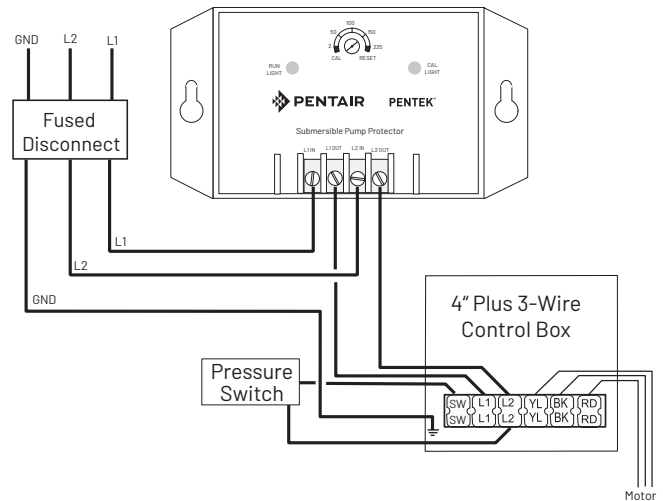
Figure 11-2: "Plus" Control Box Connection for SPP233
