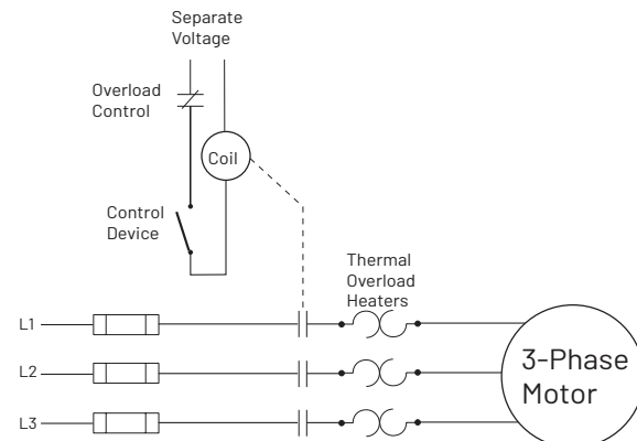
Figure 4-9: Separate Voltage Control
