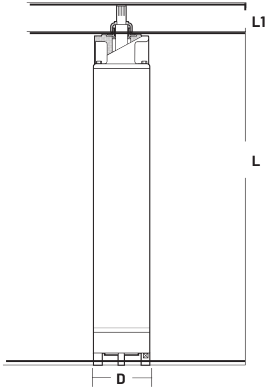
Figure 6-4: Dimensions
