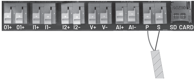
Figure 8-17: Example RS-485 Connection
