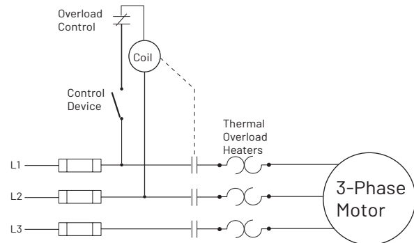
Figure 4-7: Line Voltage Control
