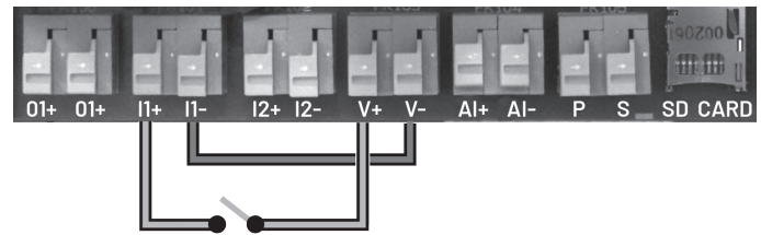
Figure 8-14: Input with Internal 24 Volt Supply
