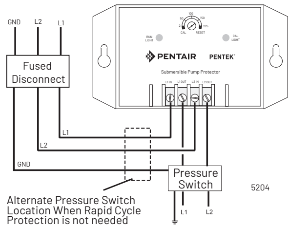
Figure 11-3: Two-Wire Connection for SPP233
