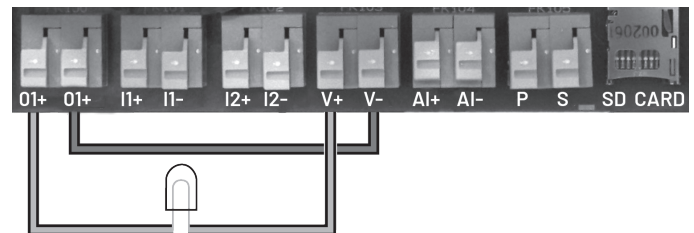
Figure 8-16: Output Relay with Internal 24 Volt Supply
