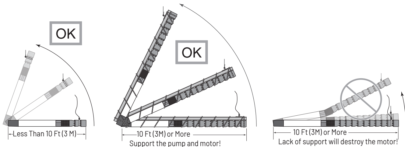
Figure 6-1: When the pump and motor together (without any riser pipe) are 10ft (3m) long or more, support the assembly before lifting to avoid bending it in the middle. Never try to lift the motor or pump by the motor cables.
