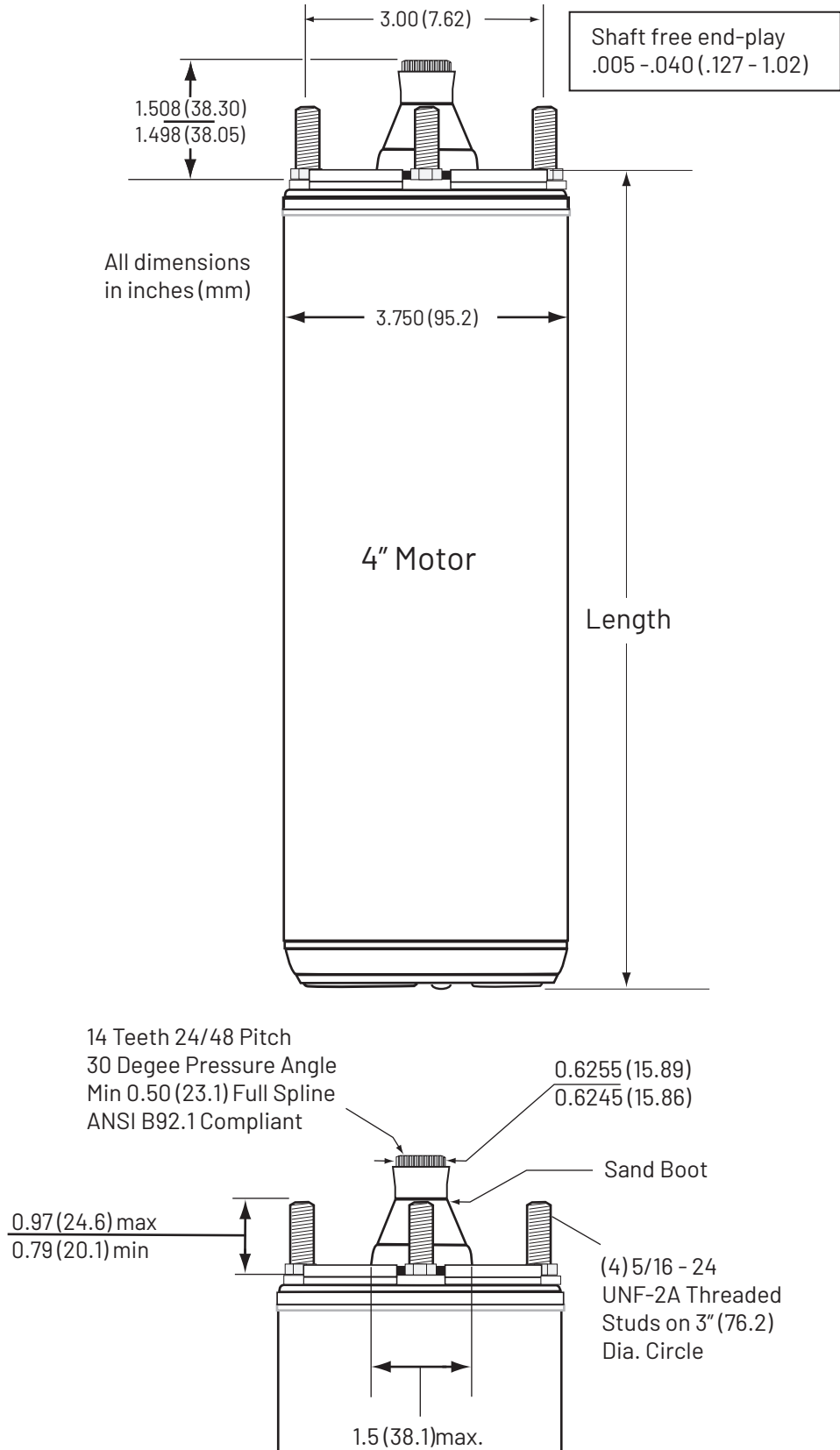
Figure 5-1: Single and Three Phase XE Series 4" Motor Dimensions
