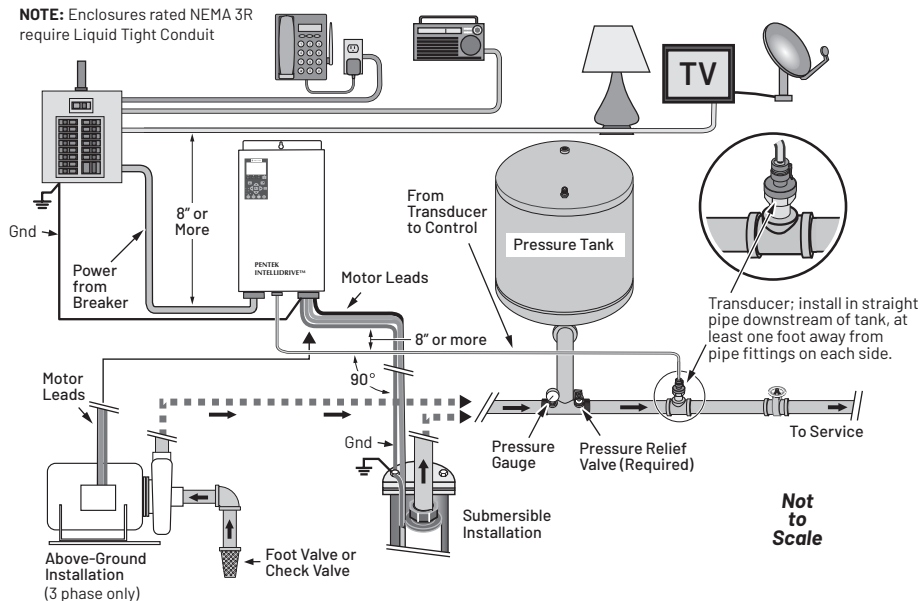
Figure 8-1: A typical residential installation layout
