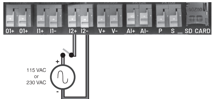
Figure 8-15: External Input with External Supply
